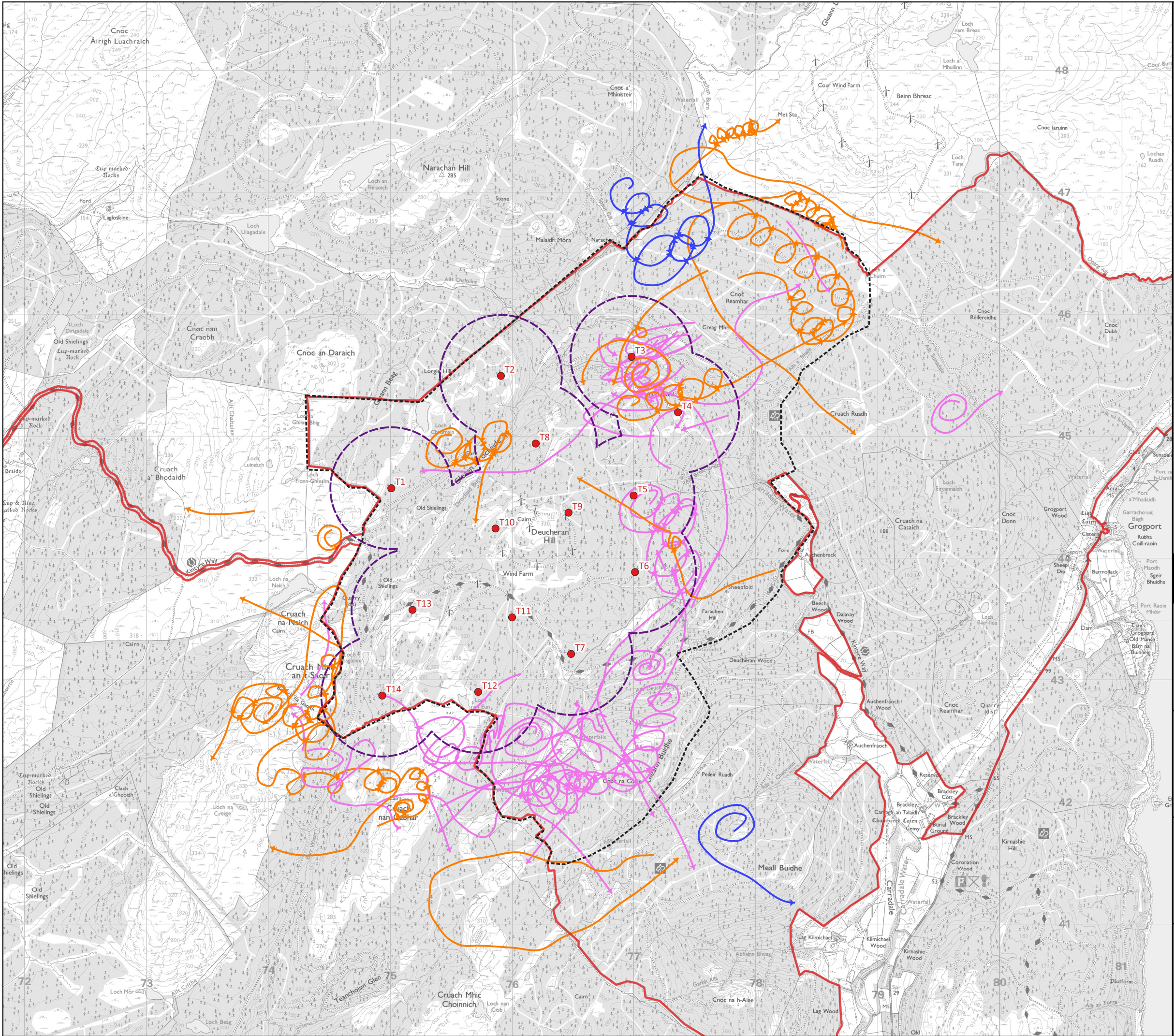
Figure 8.4a: VP flight activity surveys - Raptors (Year 2)
